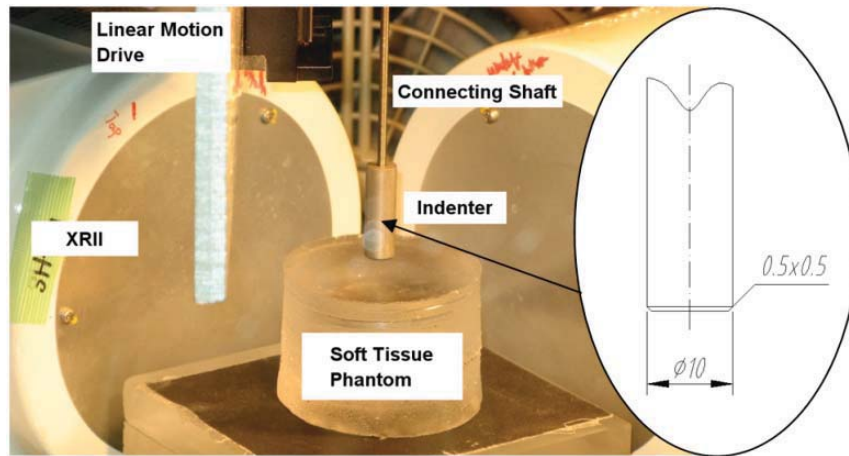
Fig. 1. Experiment setup of soft tissue phantom (height of 46 mm, diameter of 64 mm, and layer thickness of 9 mm) indentation and indenter geometry.
