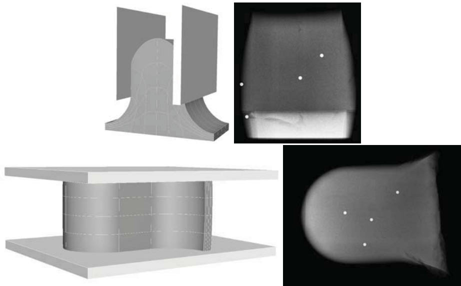
Fig. 3. The gel phantom in the two compressed states. Model and x-ray image pairs illustrating the CC-like (top pair) and ML-like (bottom pair) compressions that were applied to the gel phantom to image the metal beads embedded within the gel.
