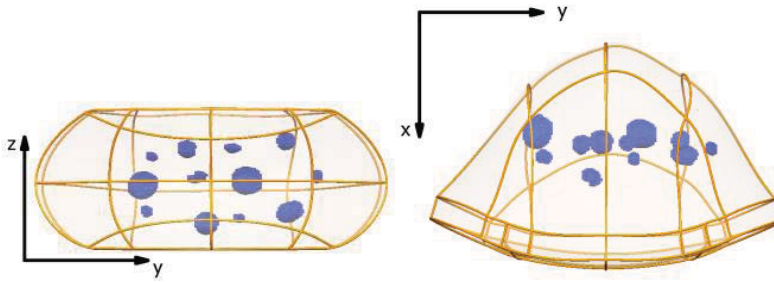
Fig. 4. The breast phantom contained twelve internal masses. The locations of these lesions when the phantom was compressed were predicted using the biomechanical model.
