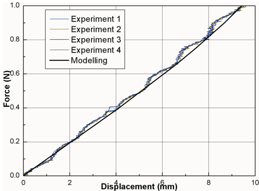
Fig. 5. Soft tissue phantom indentation: comparison of modelling and experimental results in force magnitude.
