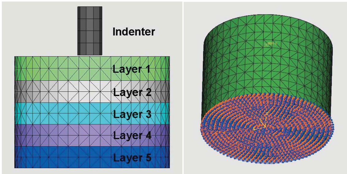
Fig. 4. Soft tissue phantom mesh (left). The nodes defining the bottom surface were rigidly constrained in the model (right).
