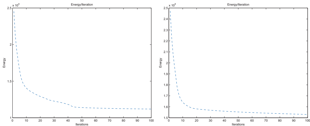
Fig. 8. Energy decrease versus iterations for the proposed multilayer segmentation models, validating the numerical stability of the algorithm: multilayer model without atlas (left), multilayer model with atlas (right).
