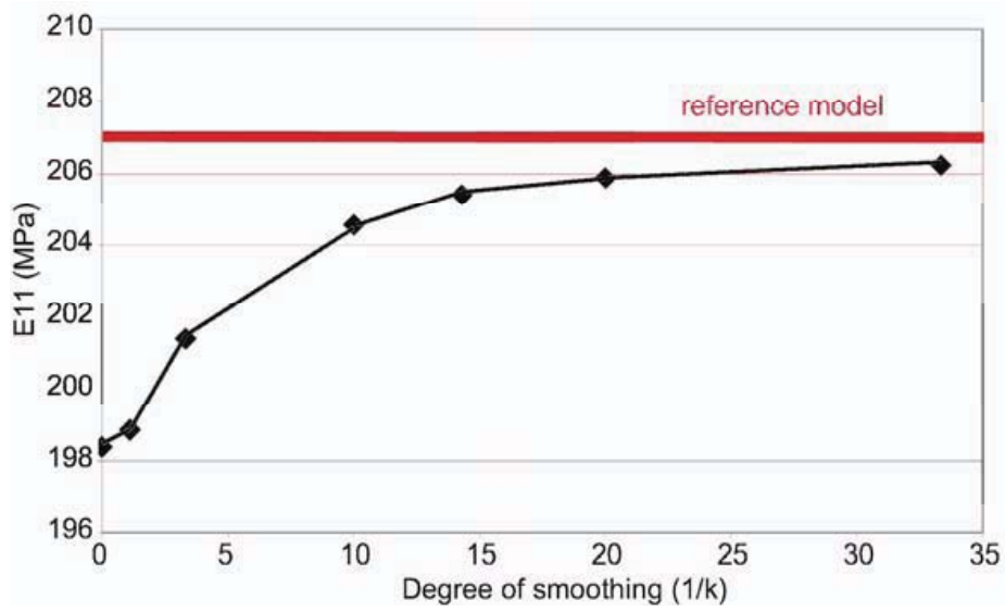
Fig. 3. Evolution of the apparent Young's modulus in the X direction for the 16µm model with different degrees of smoothing.
