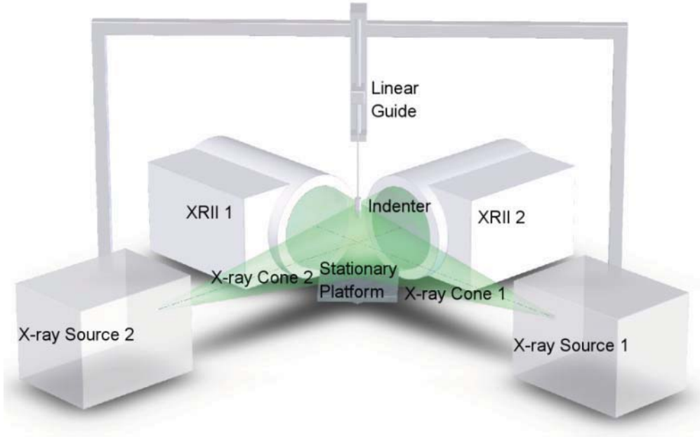
Fig. 2. Setup of the custom-built bi-plane XRII system
