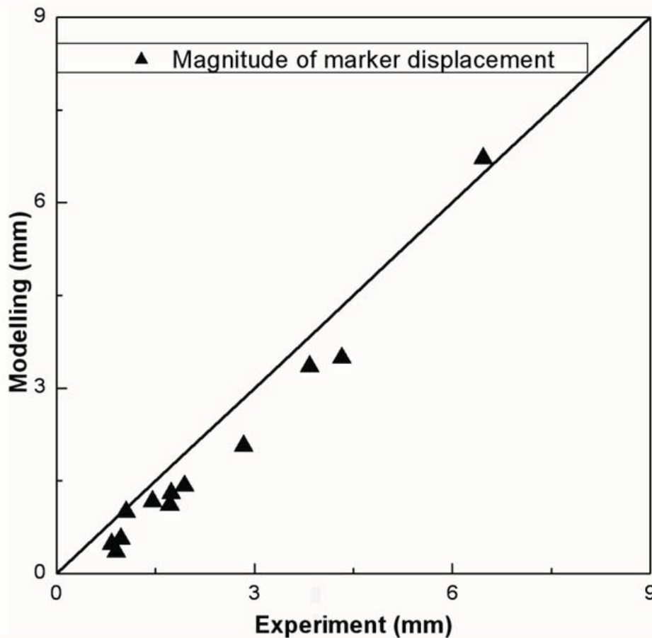
Fig. 7. Soft tissue phantom indentation: the correlation of the predicted and measured magnitude of marker displacements magnitude. Horizontal axis - experimentally determined magnitude. Vertical axis - magnitude predicted by the model summarised in Fig. 4. The data points scatter along a 45° line, which indicates that the predicted and measured results are linearly correlated.
