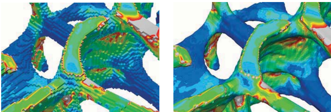
Fig. 5. Details of the Mises stress in the trabecular structure generated (left) without smoothing and (right) with smoothing.
