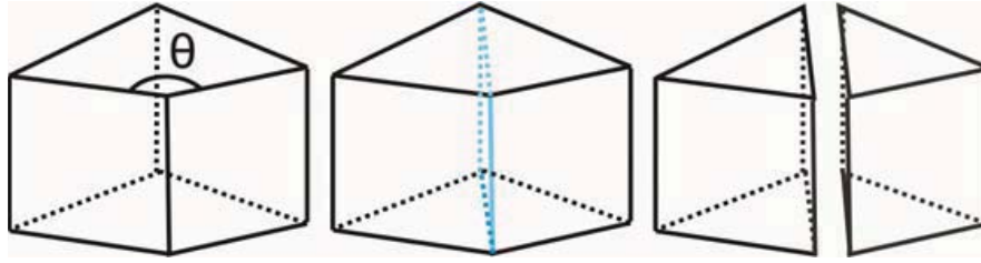
Fig. 2. Correction of elements featuring large angles (here represented by \theta ). The elements are divided into two prism elements along the plane that passes through the “large angle” edge.
