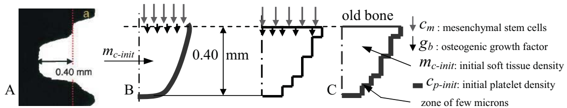
Fig. 1. Wound compartment (A, reproduced from [8]), idealized (B) and further simplified (C, used for the simulations) geometrical domain, showing initial and boundary conditions. The thick zone of 5 \mu\text{m} in which the surface-specific parameter values were applied is shown as well (C).
