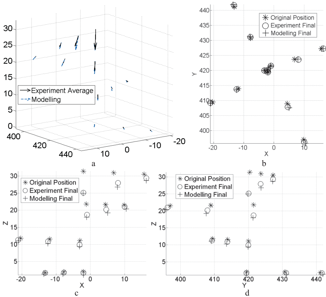
Fig. 6. Soft tissue phantom indentation: (a) Comparison of predicted and measured marker displacements at the indentation depth of 10 mm. (b), (c), (d) Comparisons of the computed and experimental final positions of the markers at the indentation depth of 10 mm in XY, XZ, YZ plane. Original marker positions are included to indicate the magnitude of displacement.
