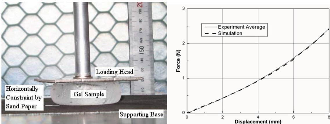
Fig. 3. The gel samples were tested by semi-confined uniaxial compression (left). The material constants were determined by calibrating the model of the compression test setup to the experiment average force-displacement relations using ABAQUS finite element solver.
